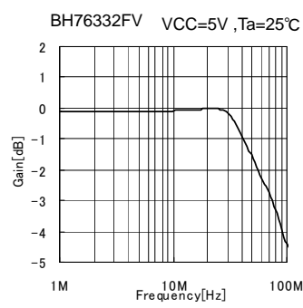
Fig.79 Frequency Response
