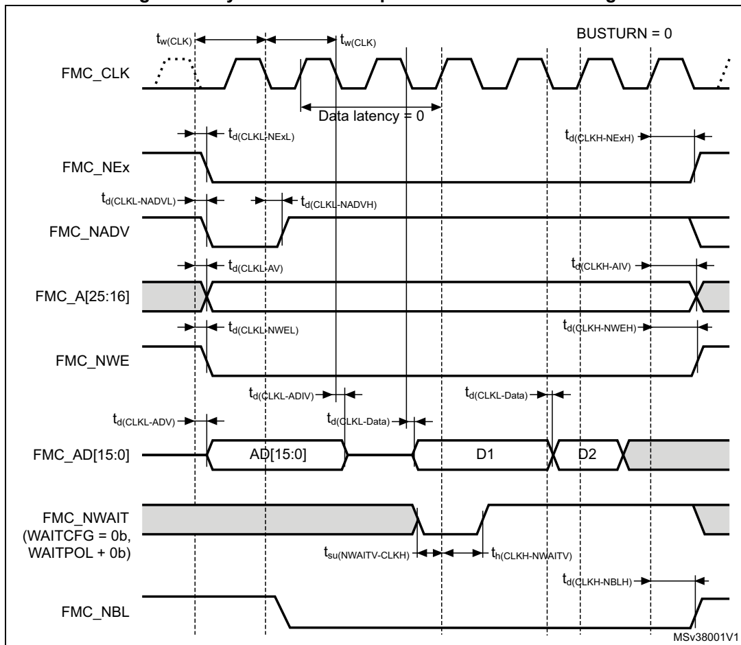
Figure 47. Synchronous multiplexed PSRAM write timings
