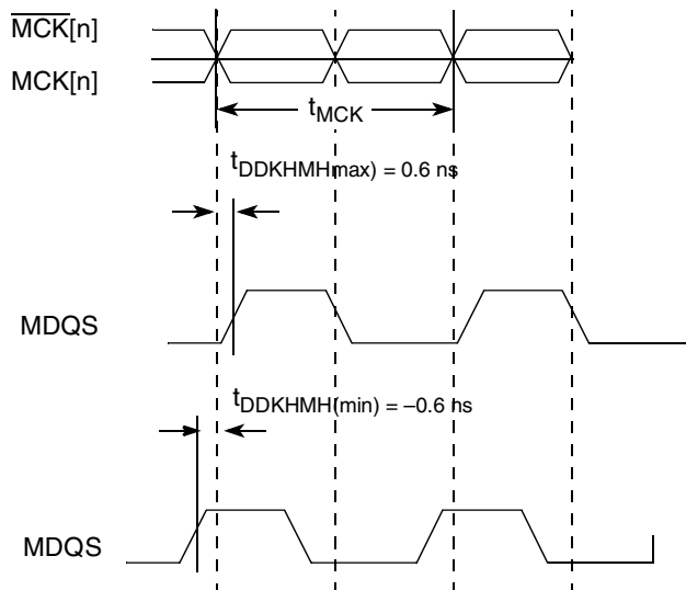
Figure 5. Timing Diagram for t_{\text{DDKMHM}}
