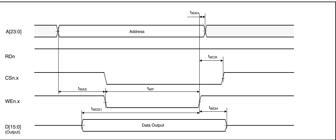
Figure 29. Write cycle timing: 16-bit write on 16-bit memory
