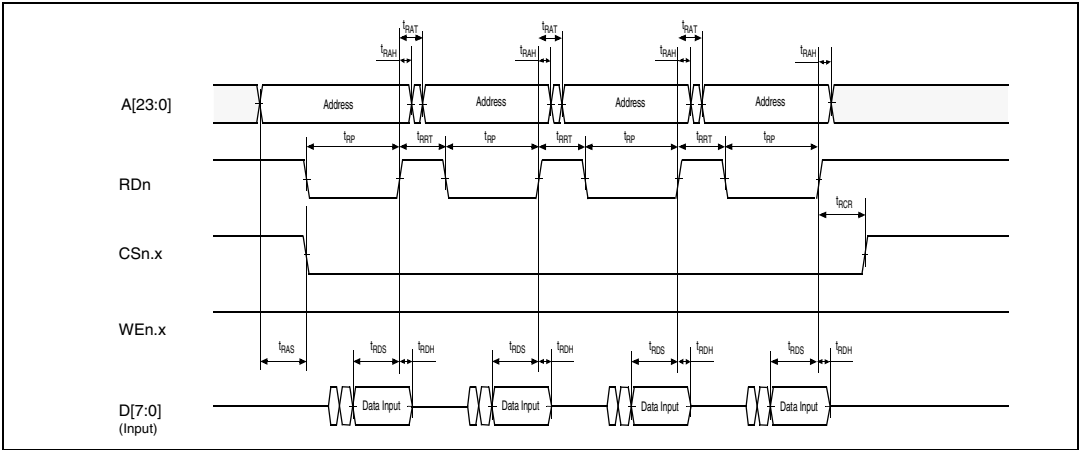
Figure 28. Read cycle timing: 32-bit read on 8-bit memory
