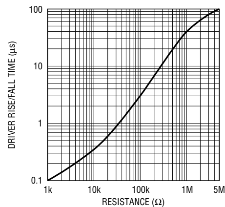
Figure 29. V.10 Driver Rise and Fall Time vs Resistor Value
