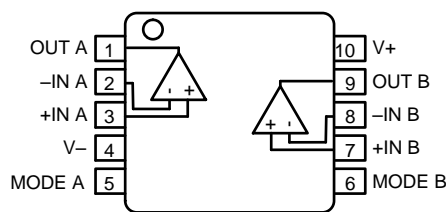
OPA2625: DGS Package 10-Pin VSSOP Top View
