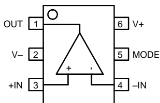
OPA625: DBV Package 6-Pin SOT Top View
