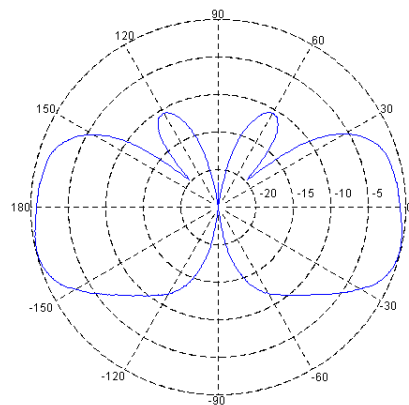
Elevation (E-field) radiation pattern
