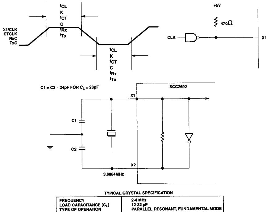
Figure 5. Clock Timing
