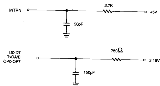
Figure 11. Test Conditions on Outputs
