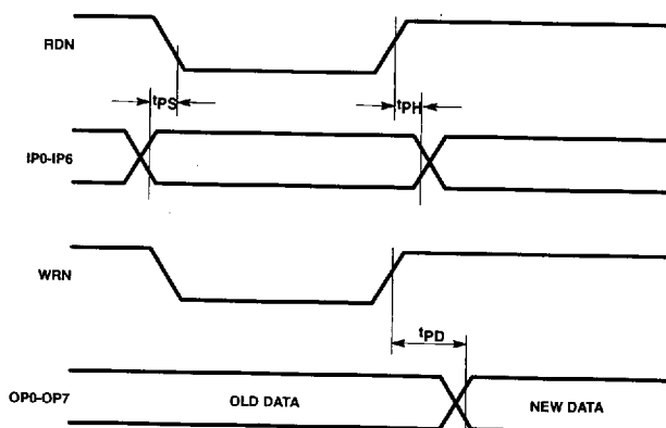
Figure 3. Port Timing
