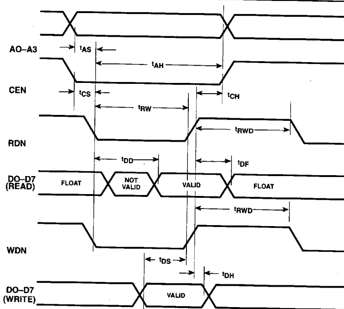
Figure 2. Bus Timing
