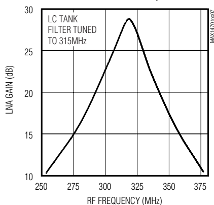
LNA GAIN vs. RF FREQUENCY
