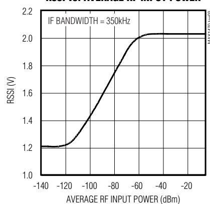
RSSI vs. AVERAGE RF INPUT POWER
