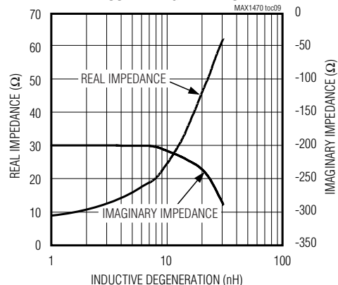
INPUT IMPEDANCE vs. INDUCTIVE DEGENERATION
