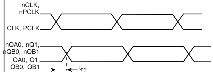
PROPAGATION DELAY
