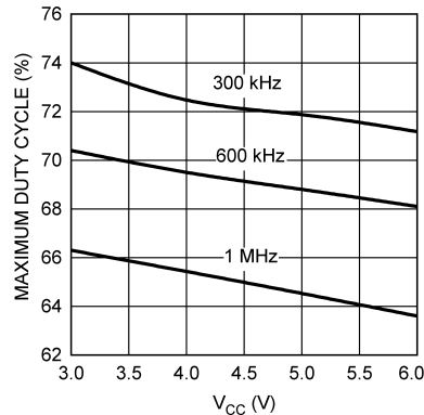
Figure 34. Maximum Duty Cycle vs V_{CC} T_J = 125^\circ\text{C}
