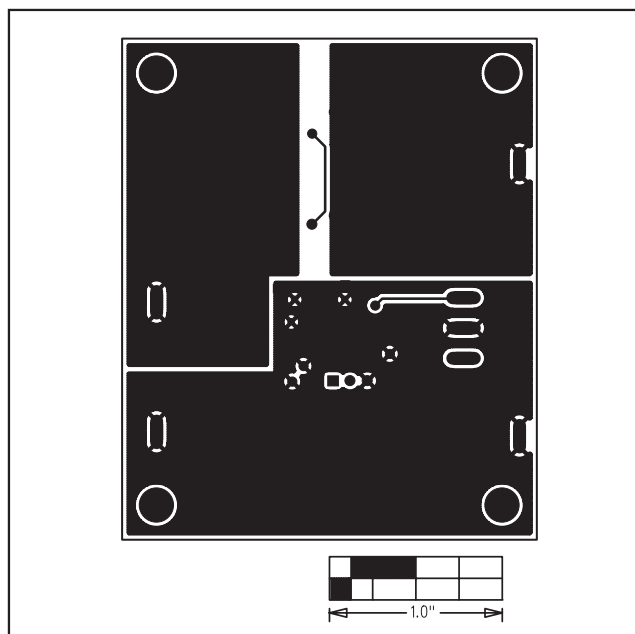
Figure 4. MAX8536 EV Kit PCB Layout—Solder Side
