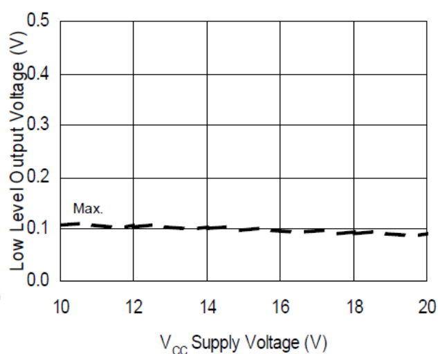
Figure 11B. Low Level Output vs. Supply Voltage
