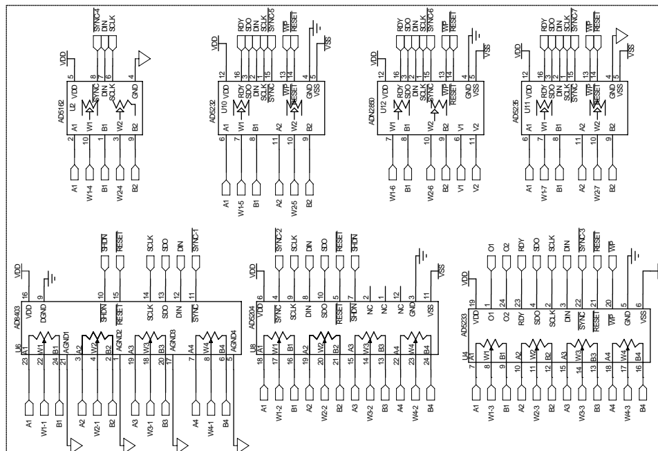
Figure 12. Schematic of Multiboard Digital Potentiometers
