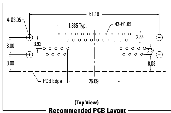
(Top View) Recommended PCB Layout
