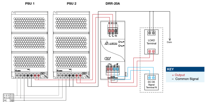
Fig. 3 Redundancy Operation Connection Diagram
