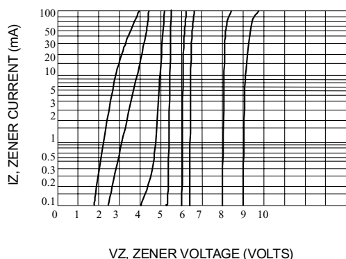
Fig. 6-VZ = 3.9 THRU 10 VOLTS
