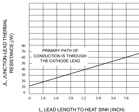
Fig. 9-TYPICAL THERMAL RESISTANCE
