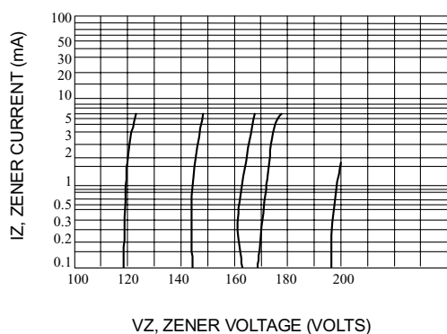
Fig. 8-VZ = 100 THRU 200 VOLTS
