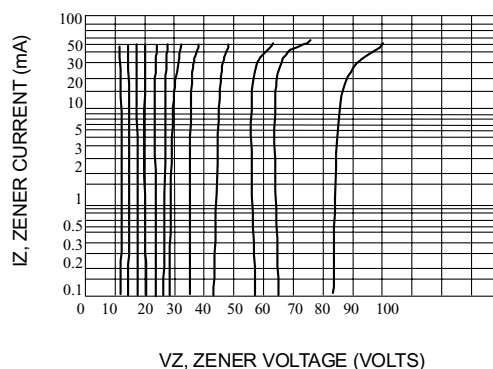
Fig. 7-VZ = 12 THRU 82 VOLTS
