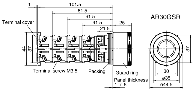
Mushroom with full guard (35mm dia. metal nut)
