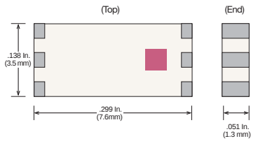
Case 44-1
