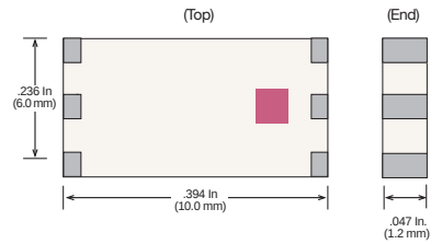
Case 51-1
