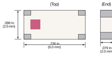
Case 43-3
