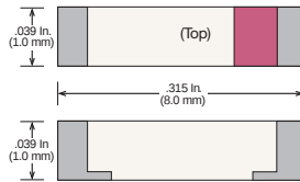
Case 44-2
