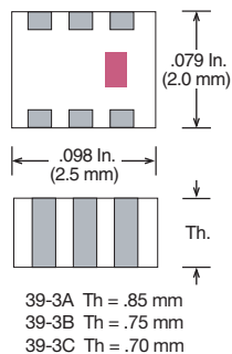
Case 39-3 (2520)
