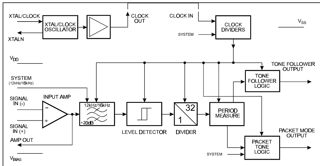
Figure 1: Block Diagram
