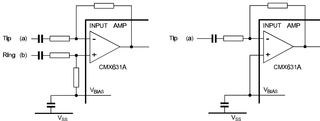
Figure 7: Input Configurations
