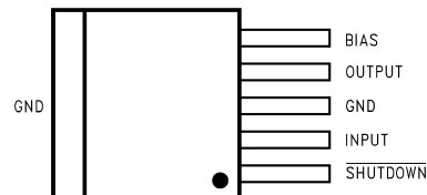
Figure 2. 5-Pin DDPAK/TO-263, Top View See KTT0005B Package
