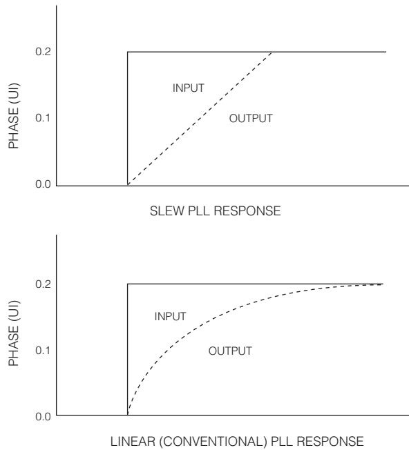
Fig. 14 PLL Characteristics
