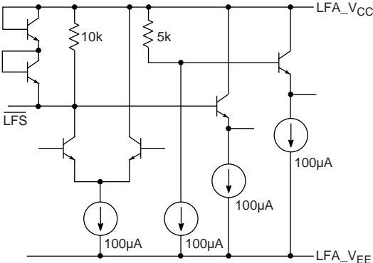
Fig. 6 LFS Input Circuit
