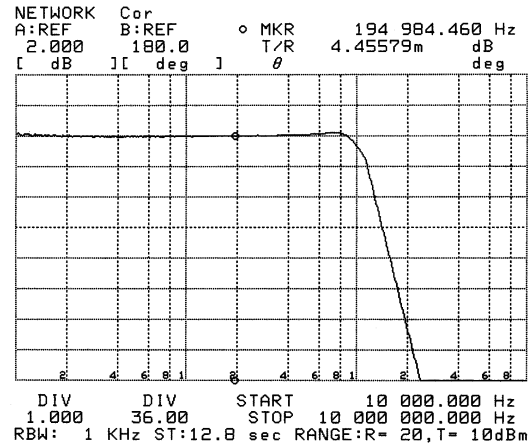
Fig. 18 Typical Jitter Transfer Curve at Setting A in Table 2
