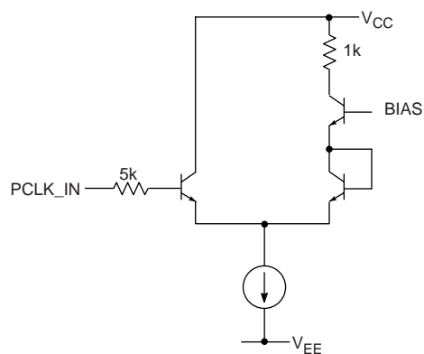
Fig. 11 PCLK_IN Circuit
