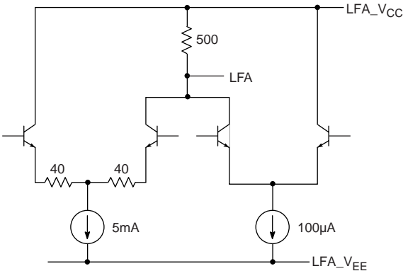
Fig. 4 LFA Circuit
