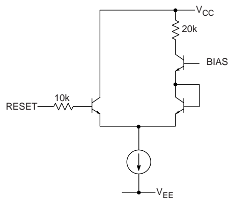
Fig. 12 RESET Circuit
