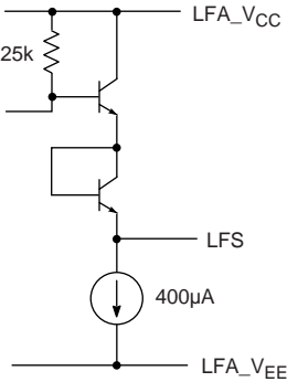
Fig. 5 LFS Output Circuit
