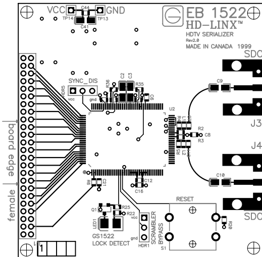
Fig. 28 Top Layer of EB1522 PCB Layout
