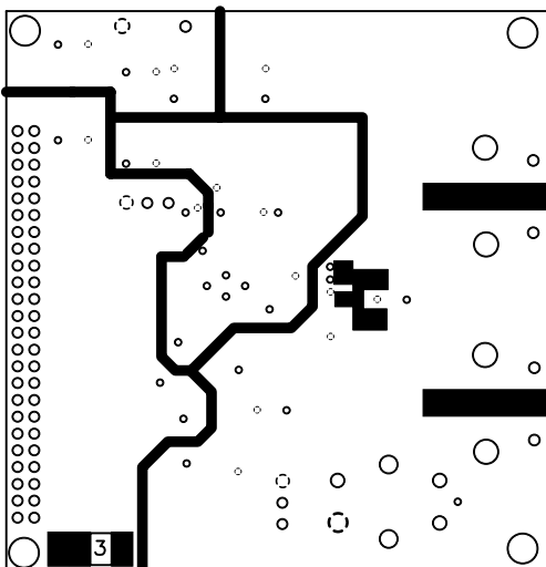
Fig. 30 Power Layer of EB1522 PCB Layout
