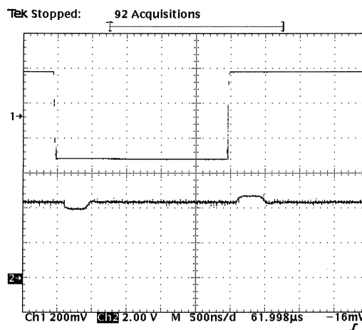
Fig. 22 Jitter Demodulation Signal
