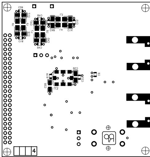
Fig. 31 Bottom Layer of EB1522 PCB Layout
