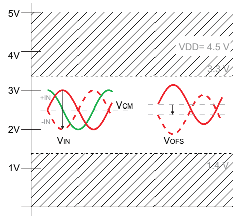
Figure 3: Permissible input voltage range at V_{DD} = 5\text{ V} \pm 10\% .
