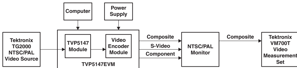
Figure 1-5. TVP5147EVM System Level Block Diagram
