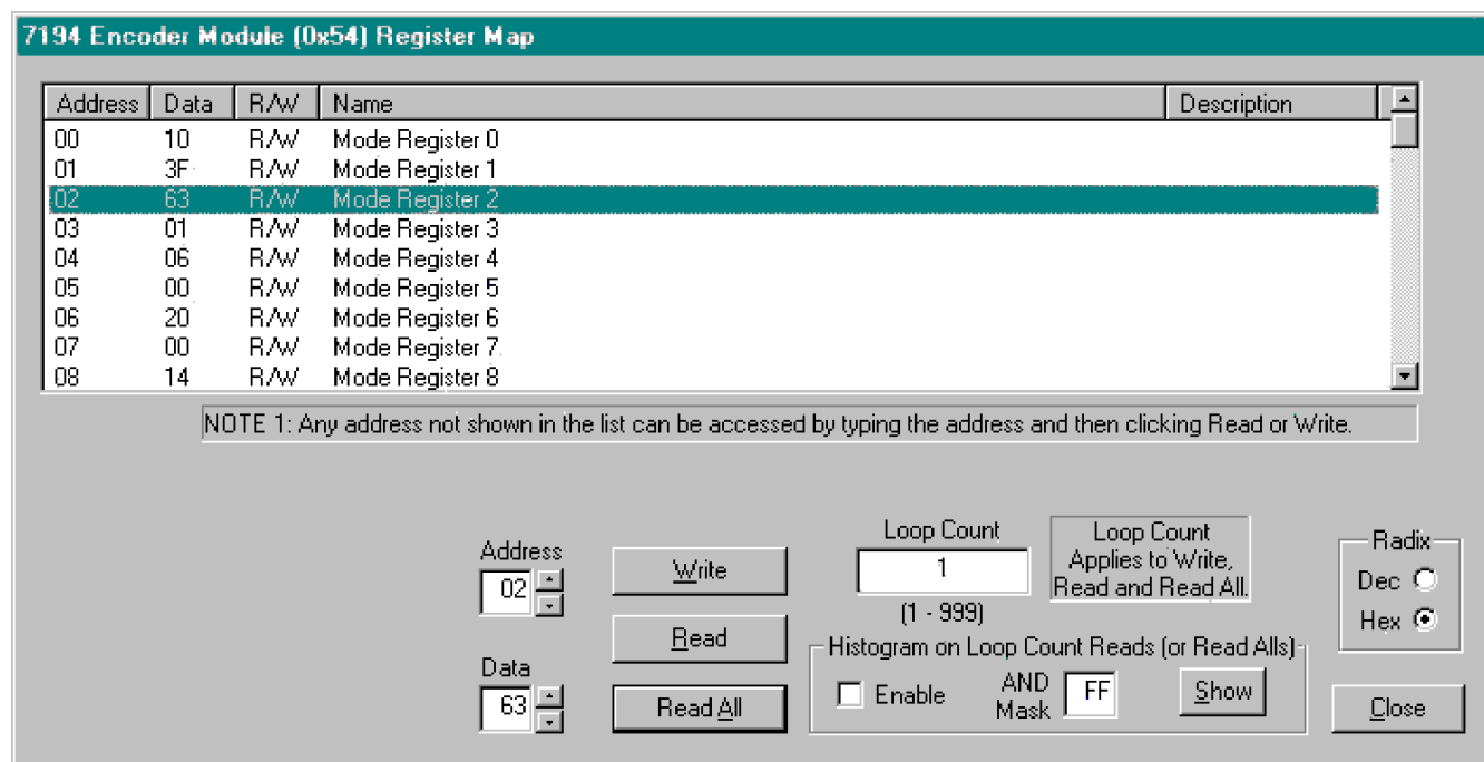
Figure 3-8. Encoder Module Editor
