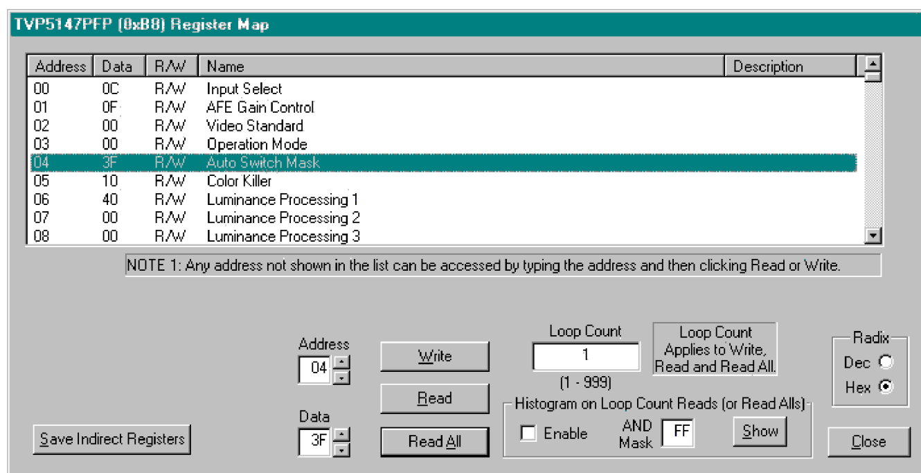
Figure 3-7. Register Map Editor
