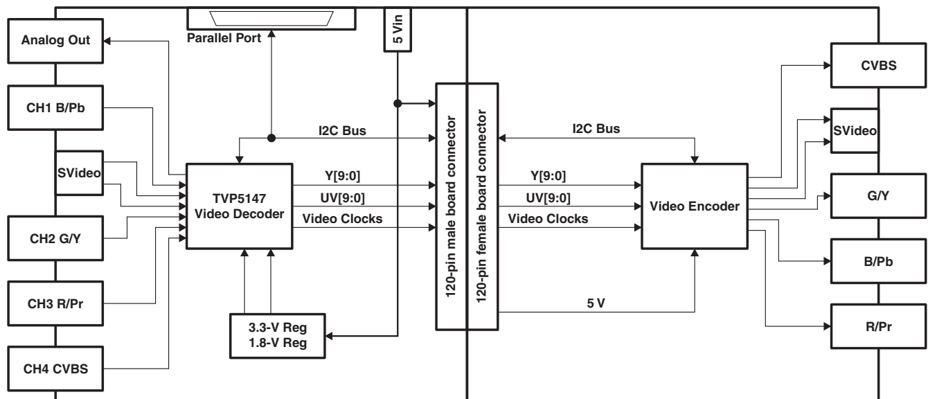
Figure 1-3. TVP5147EVM
