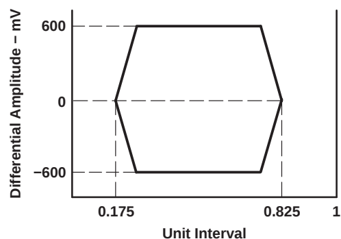
Figure 4-2. Transmit Template
