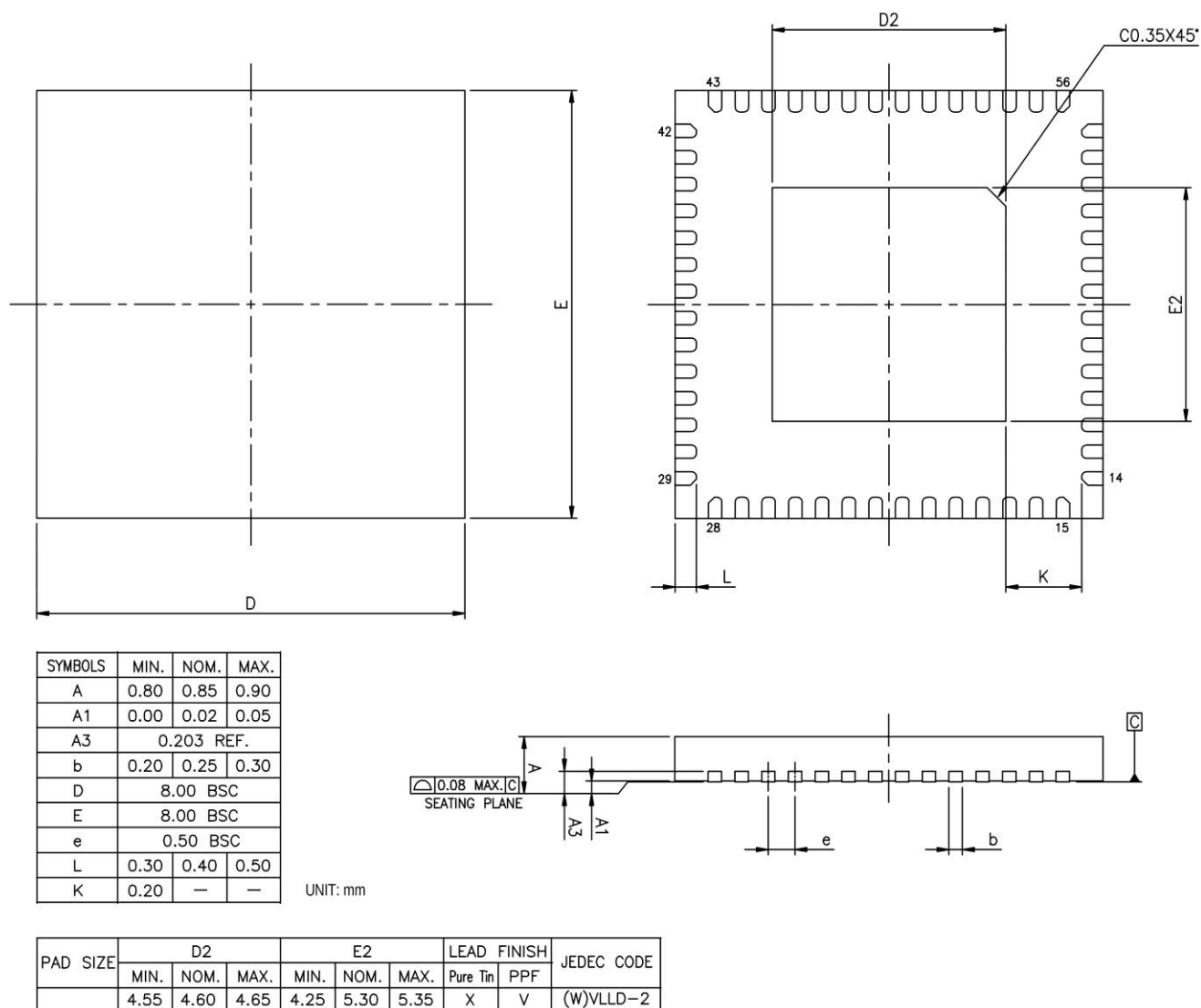
Figure 7-2 QFN-56 Package Dimensions
