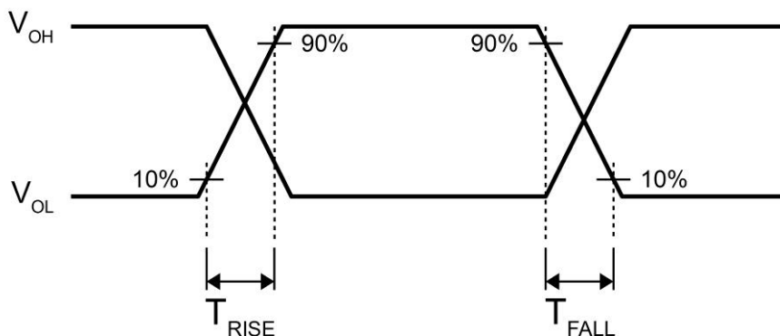
Figure 5-1 USB Rise and Fall Times for DP/DM
