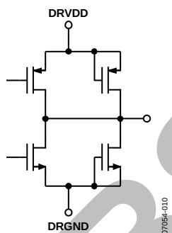
Figure 10. Digital Output
