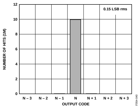
Figure 40. AD9627-11 Grounded Input Histogram
