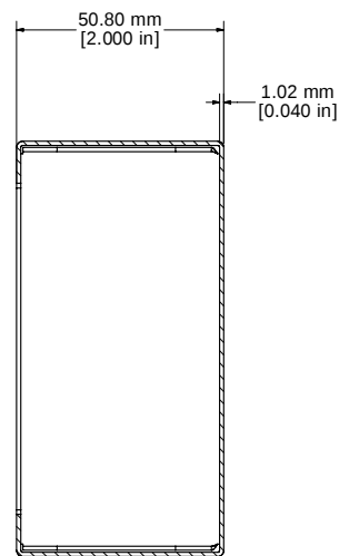
SECTION GG-GG
