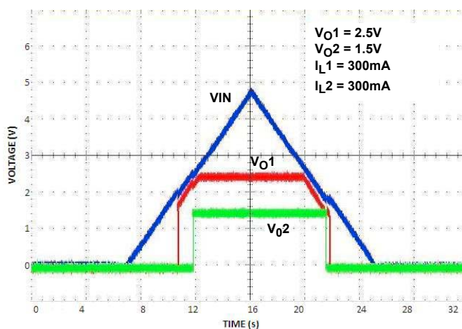
FIGURE 11. POWER-UP/POWER-DOWN
