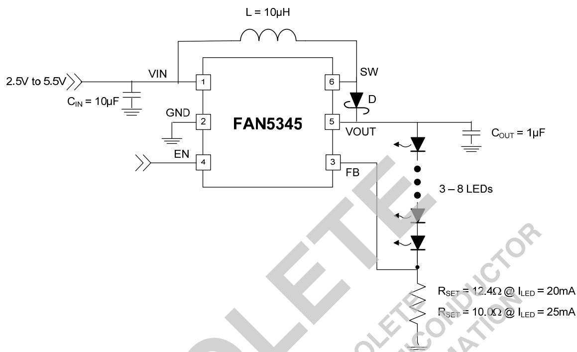
Figure 1. Typical Application
