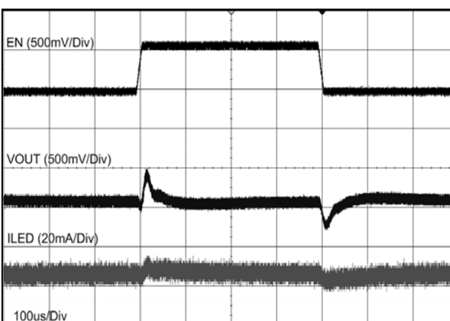
Figure 21. Line Transient Response for 7 LEDs
