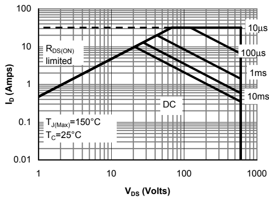
Figure 9: Maximum Forward Biased Safe Operating Area for AOT8N60 (Note F)
