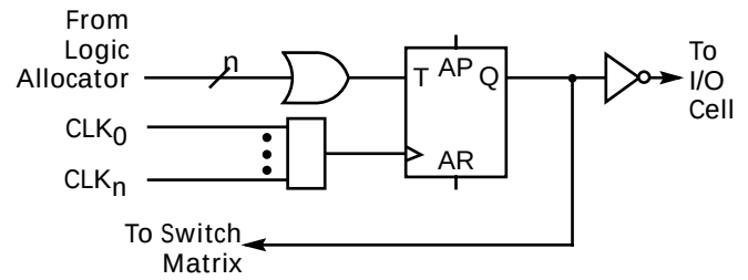
f. T-type register, active low
