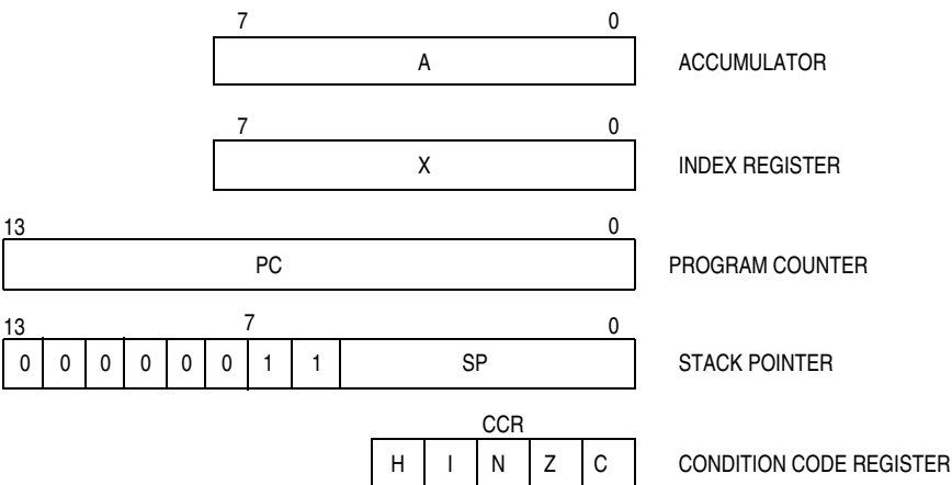
Figure 3-1. Programming Model
