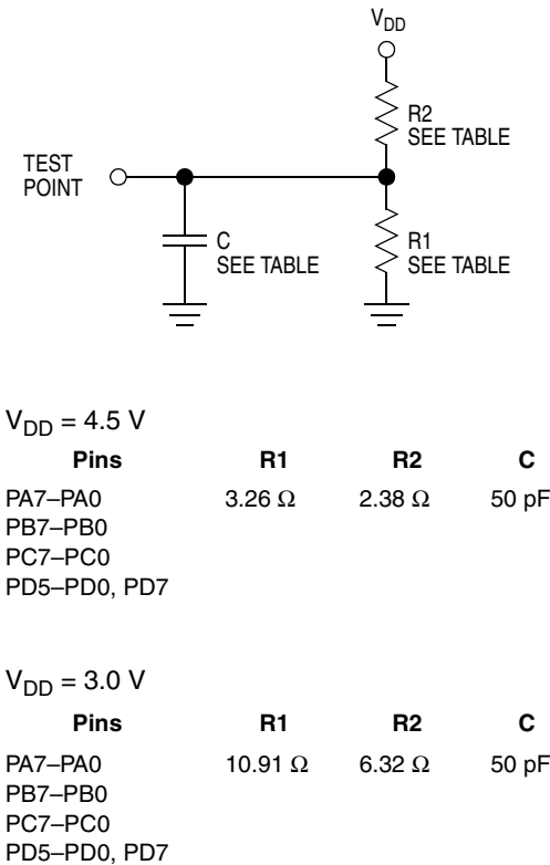
Figure 12-1. Test Load
