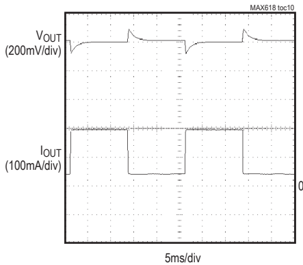
LOAD-TRANSIENT RESPONSE
