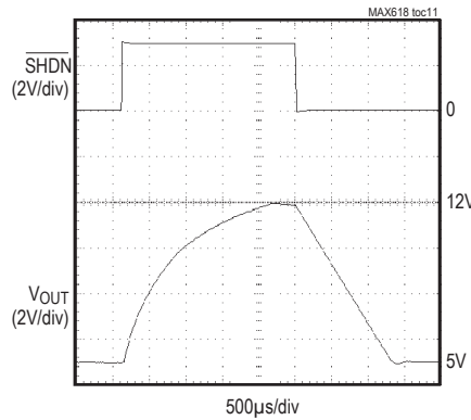
SHUTDOWN RESPONSE
