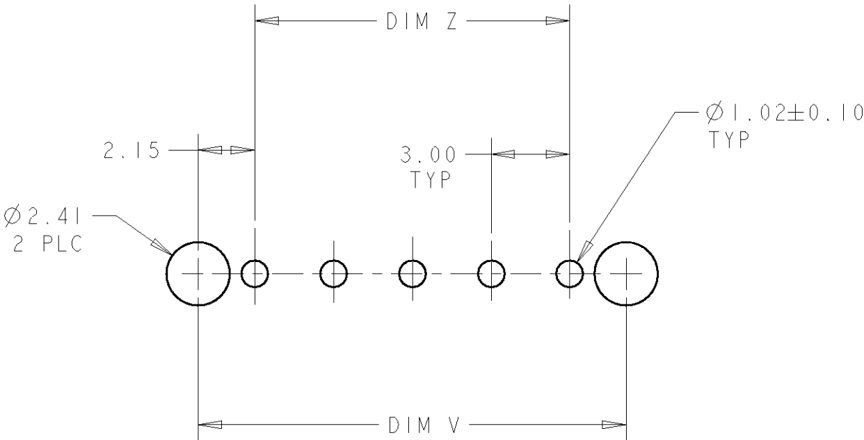
PCB LAYOUT COMPONENT SIDE 4
