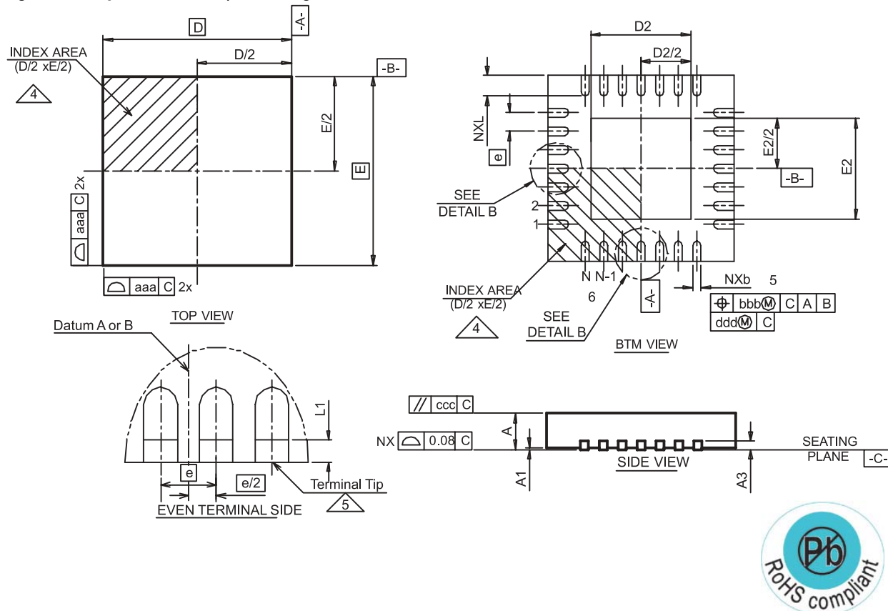
Figure 30. TQFN 3x3mm 16-pin Package
