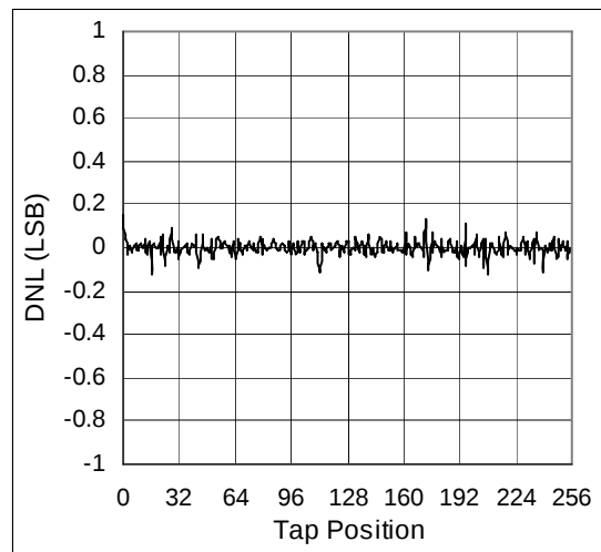
Figure 13. DNL vs. TAP Position 100k \Omega , Varistor Mode
