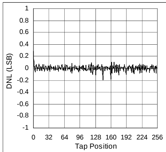
Figure 11. DNL vs. TAP Position 50k \Omega , Varistor Mode
