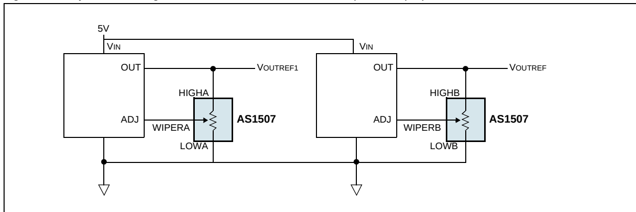
Figure 29. Adjustable Voltage Reference Circuit – V_{OUT} = 1.23V(50k\Omega/R_2(k\Omega))
