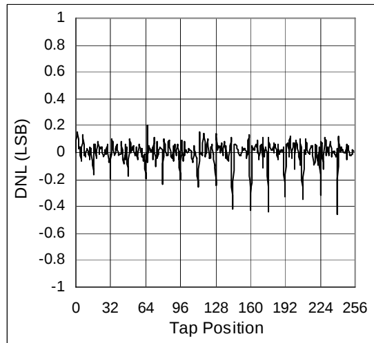
Figure 9. DNL vs. TAP Position 10k \Omega , Varistor Mode
