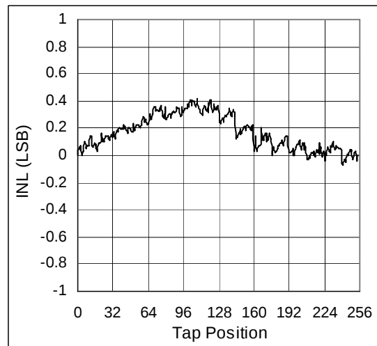
Figure 12. INL vs. TAP Position 50k \Omega , Varistor Mode
