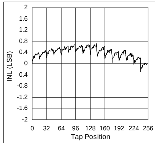
Figure 10. INL vs. TAP Position 10k \Omega , Varistor Mode
