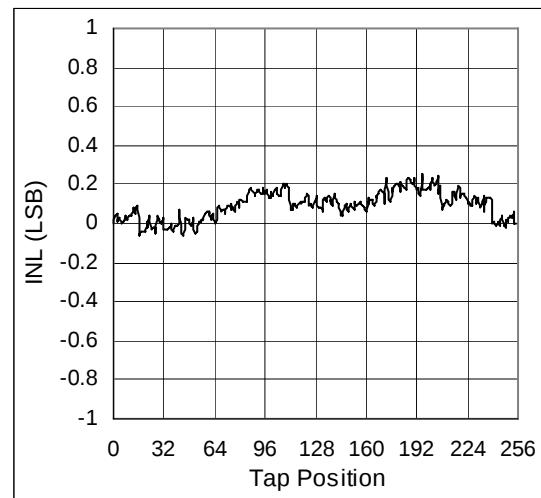
Figure 14. INL vs. TAP Position 100k \Omega , Varistor Mode
