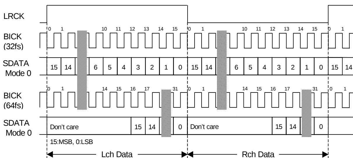
Figure 1. Mode 0 Timing
