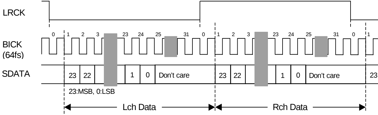
Figure 4. Mode 3 Timing
