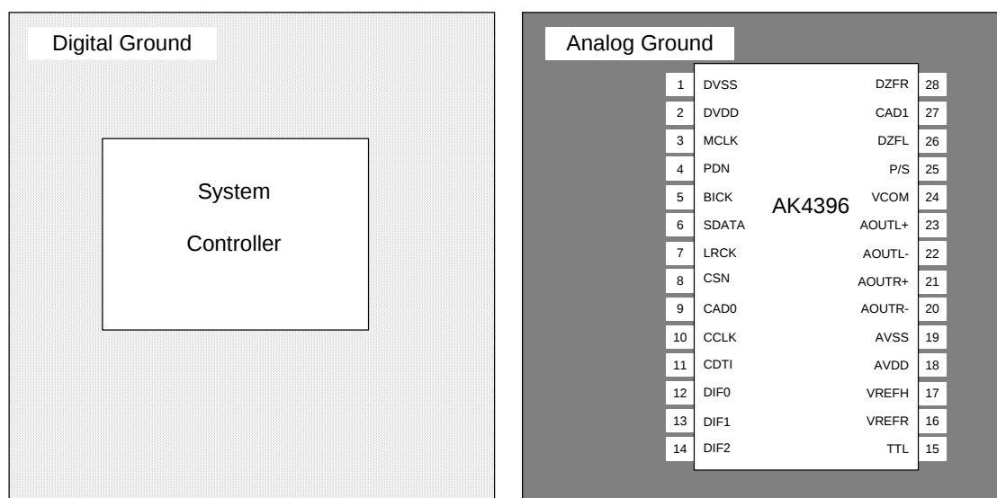
Figure 15. Ground Layout
