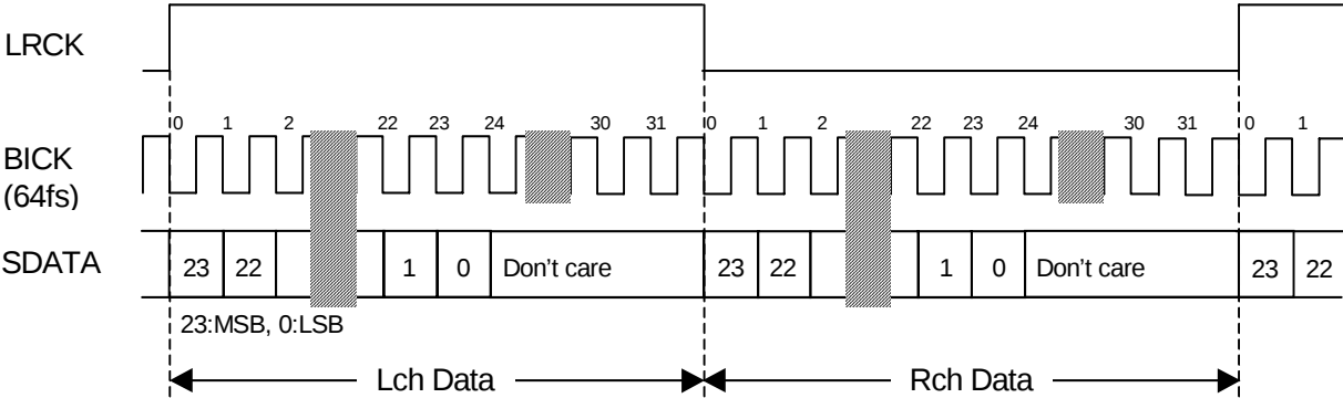
Figure 3. Mode 2 Timing
