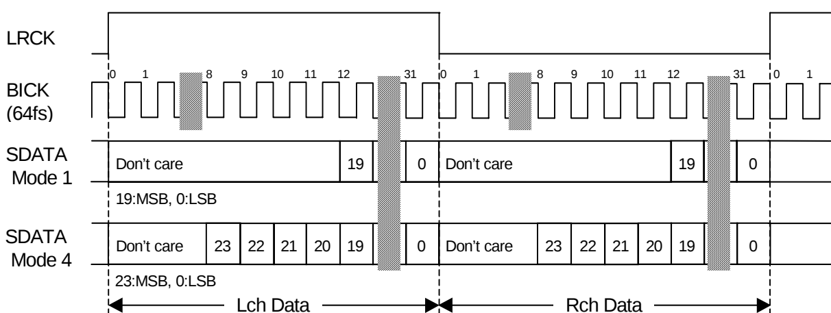
Figure 2. Mode 1, 4 Timing
