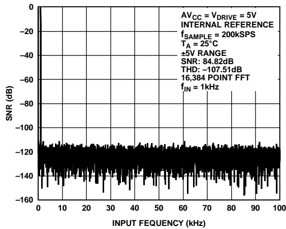
Figure 10. FFT Plot \pm 5 V Range
