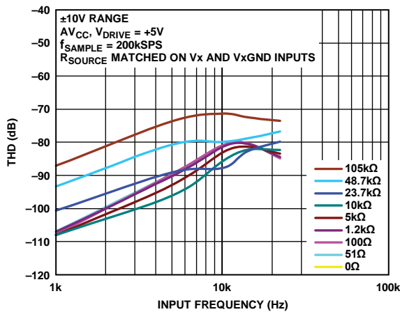
Figure 23. THD vs. Input Frequency for Various Source Impedances, \pm 10 V Range
