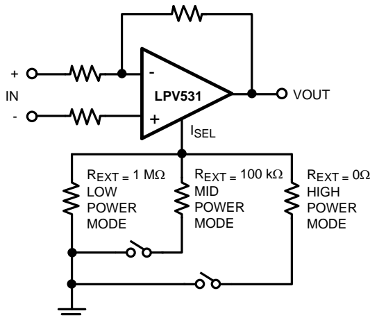
Figure 37. Power Modes Set by Resistors and Switches
