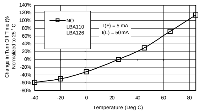
F. Turn Off Time vs. Ambient Temperature
