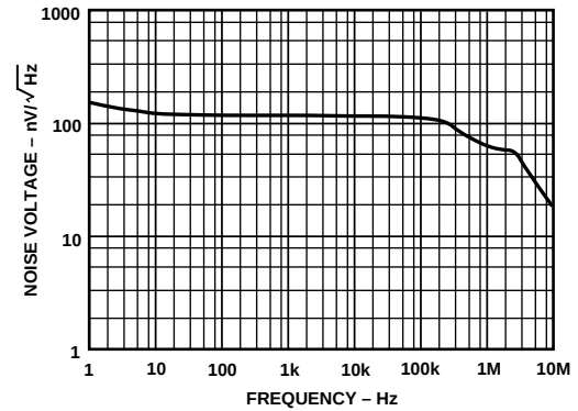
Figure 13. Reference Noise Voltage Spectral Density
