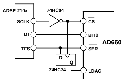
Figure 10. AD660 to ADSP-210x Interface
