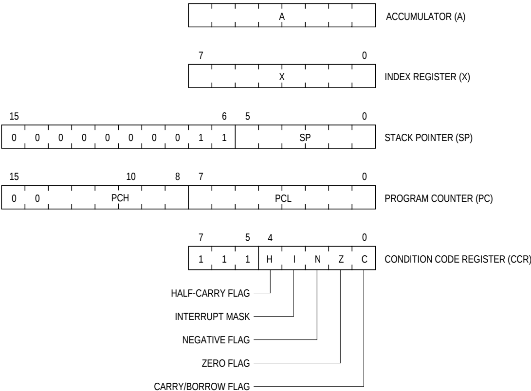
Figure 3-1. Programming Model
