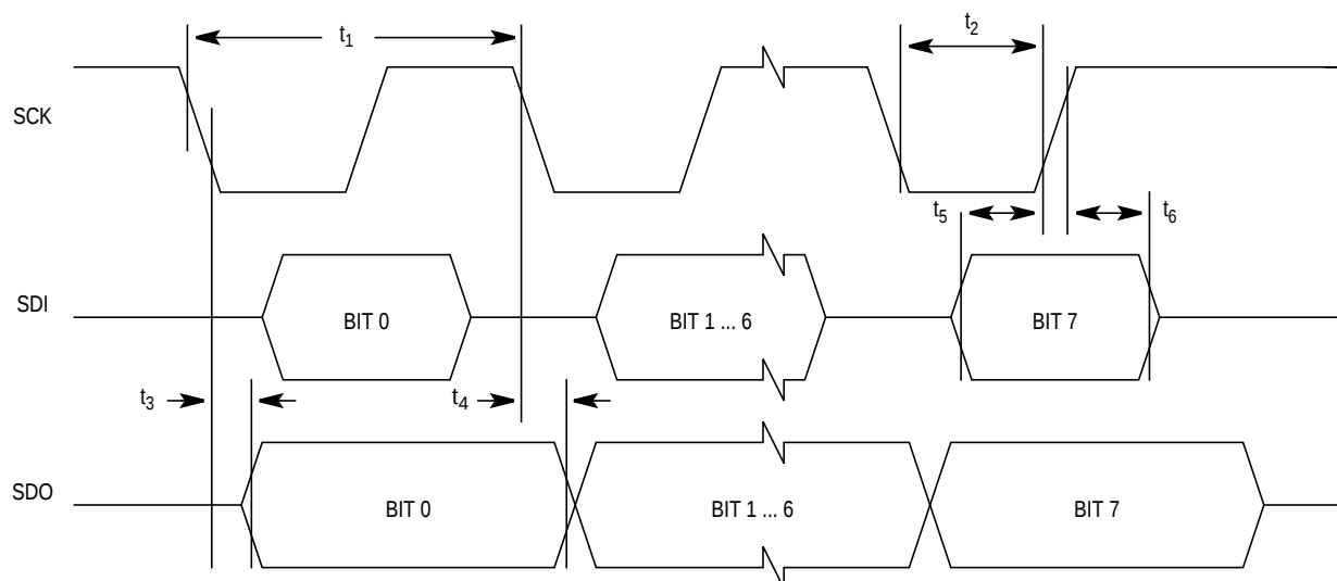
Figure 13-1. SIOP Timing Diagram
