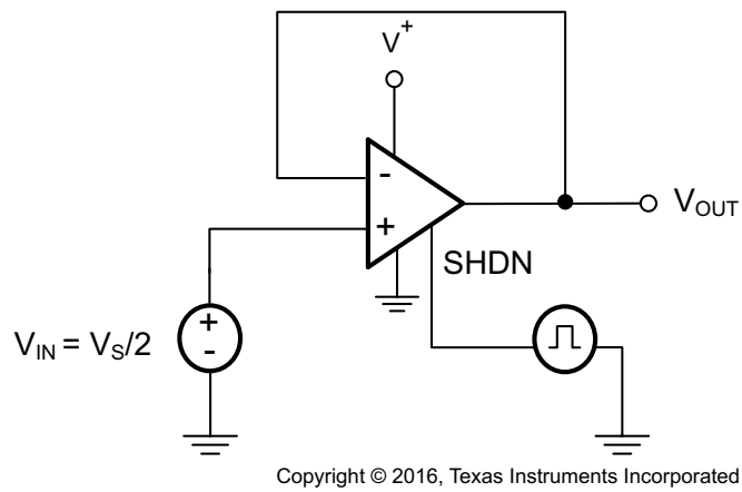
Figure 44. Turnon Time
