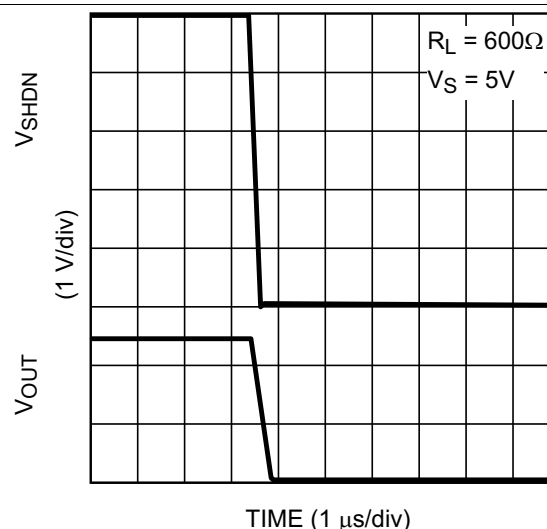
Figure 43. Turnoff Time
