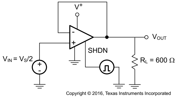
Figure 45. Turnoff Time
