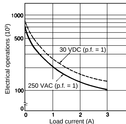
Resistive Load
