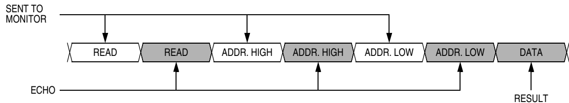
Figure 14-4. Read Transaction
