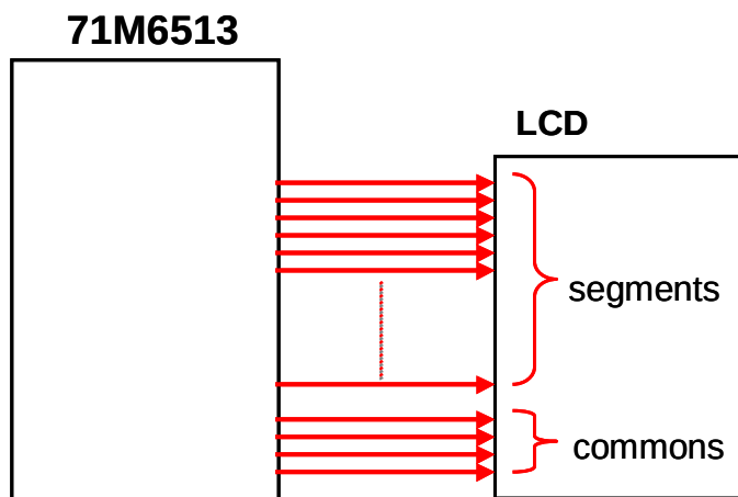
Figure 33: Connecting LCDs
