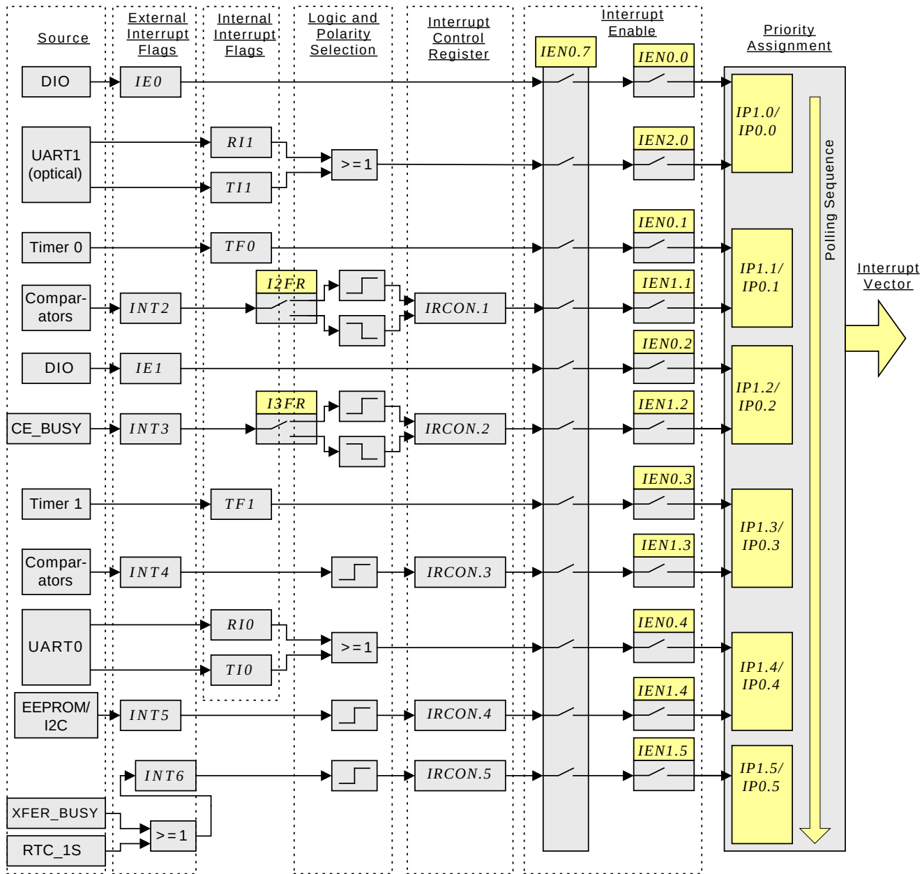
Figure 7: Interrupt Structure
