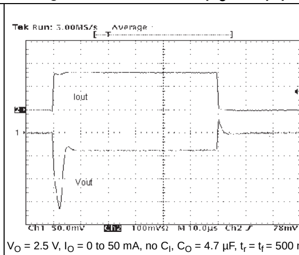
Figure 16. Load transient ( C_O = 4.7 µF)
