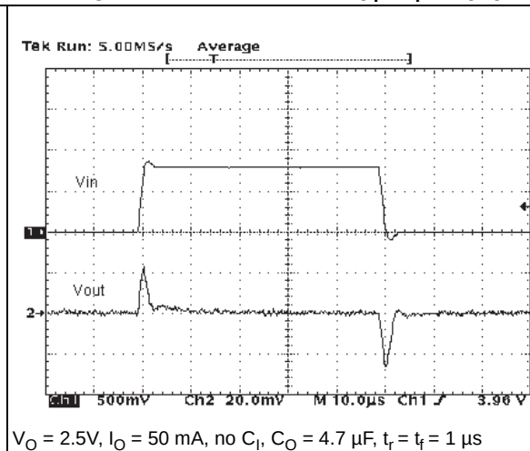
Figure 14. Line transient ( t_r = t_f = 1 µs)
