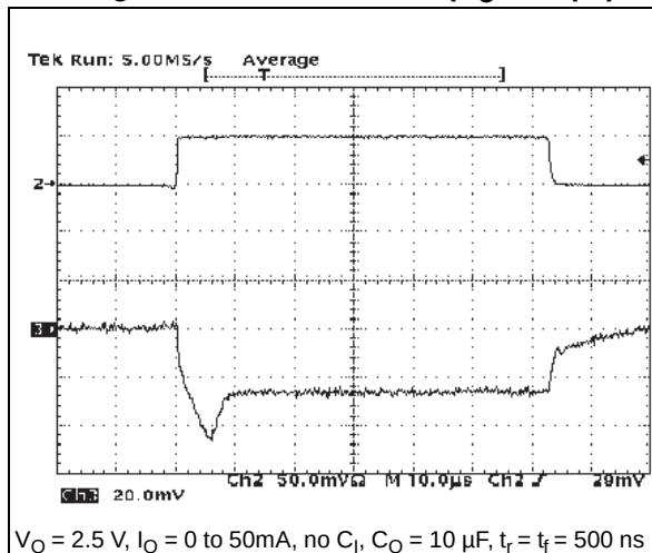
Figure 15. Load transient ( C_O = 10 µF)
