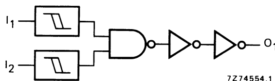
Fig.3 Logic diagram (one gate).
