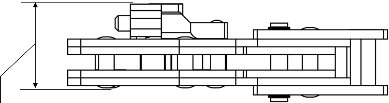
1.44" [37] CT-2525CH, CT-2550CH & CT-2500CH (WITH LOCATOR) 1.25" [32] CT-2570CH (WITHOUT LOCATOR)
