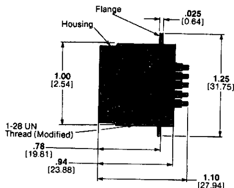
Receptacle for Hermetic Seal, Solder-Flange-Mount Part Number 862005-1
